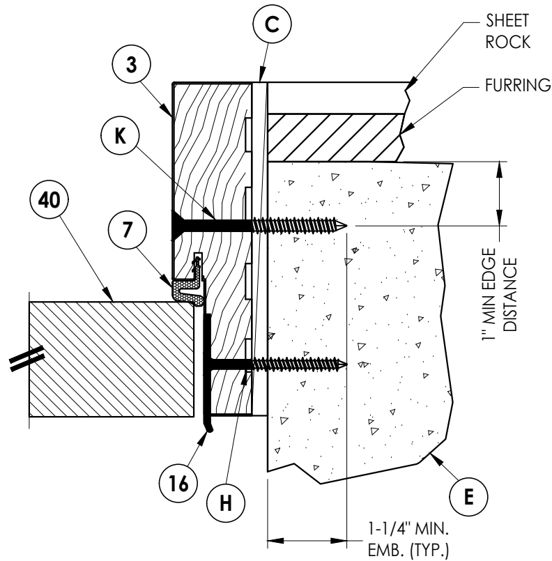
2 5 HORIZONTAL CROSS SECTION Outswing only
