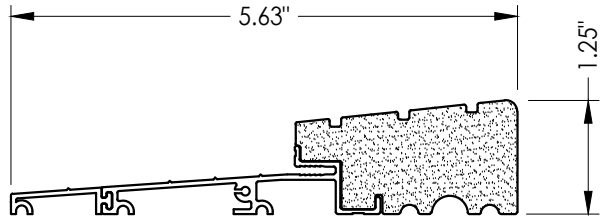
33 OUTSWING THRESHOLD w/ sill extension
