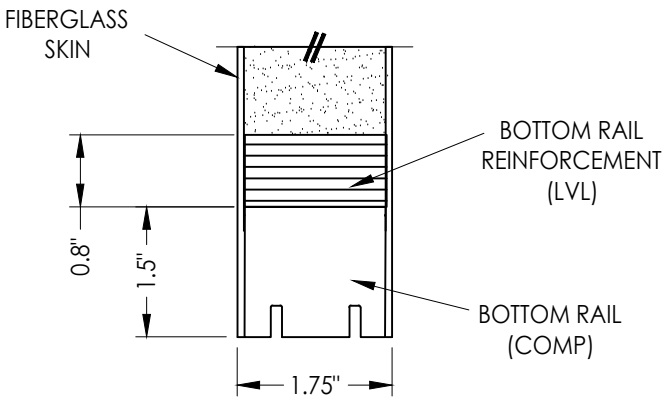
2 2 VERTICAL CROSS SECTION
