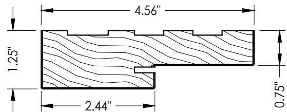
1 HEAD & JAMBS FINGER JOINT PINE
