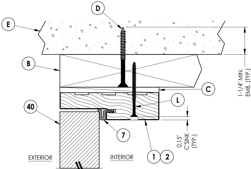
3 VERTICAL CROSS SECTION Outswing shown - Inswing also approved
