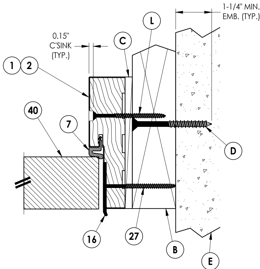
2 HORIZONTAL CROSS SECTION Outswing shown - Inswing also approved
